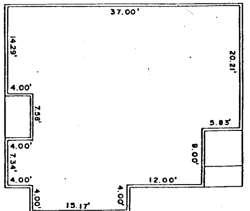
UNIT "C" SQ. FT. INTERIOR AIR SPACE 1059
