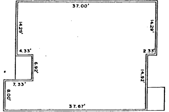
UNIT "A" SQ. FT. INTERIOR AIR SPACE 1040
